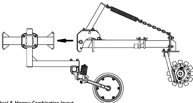
Presswheel & Harrow Combination layout
